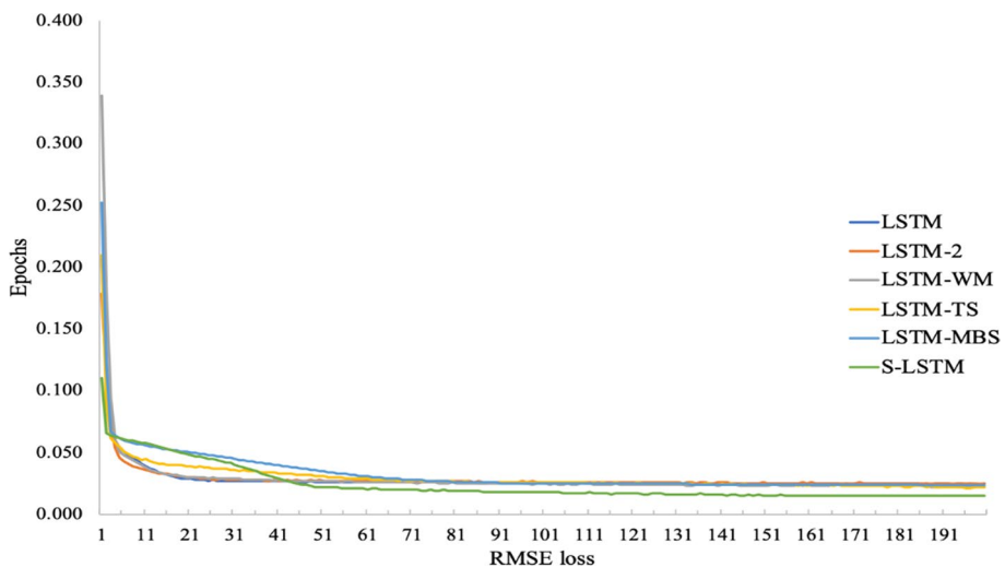
Fig. 13 Graph comparing the RMSE losses among LSTM (with 4 neurons), LSTM-2 (batch size of 2), LSTM-WM (using Window Method), LSTM-TS (with Time-Steps), LSTM-MBS (with Memory Between Batches), S-LSTM (Stacked LSTM with Memory Between Batches) over 200 epochs
